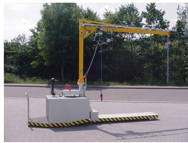
SO E 29591, EGU-5010 SO, Capacity platform 2000 kg, Capacity extension 250 kg, projection 3000 mm, swivel range 2 x 120°, hook height 2600 mm, platform lift 290 mm, fixed passenger platform
