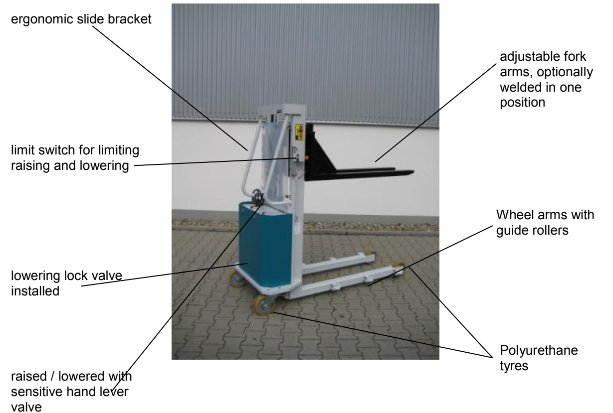
SO E 31186, E 60-1020B SO, Load capacity 600 kg at load centre distance 1000 mm, Lift height 220-1350 mm, Fork length 1300 mm
