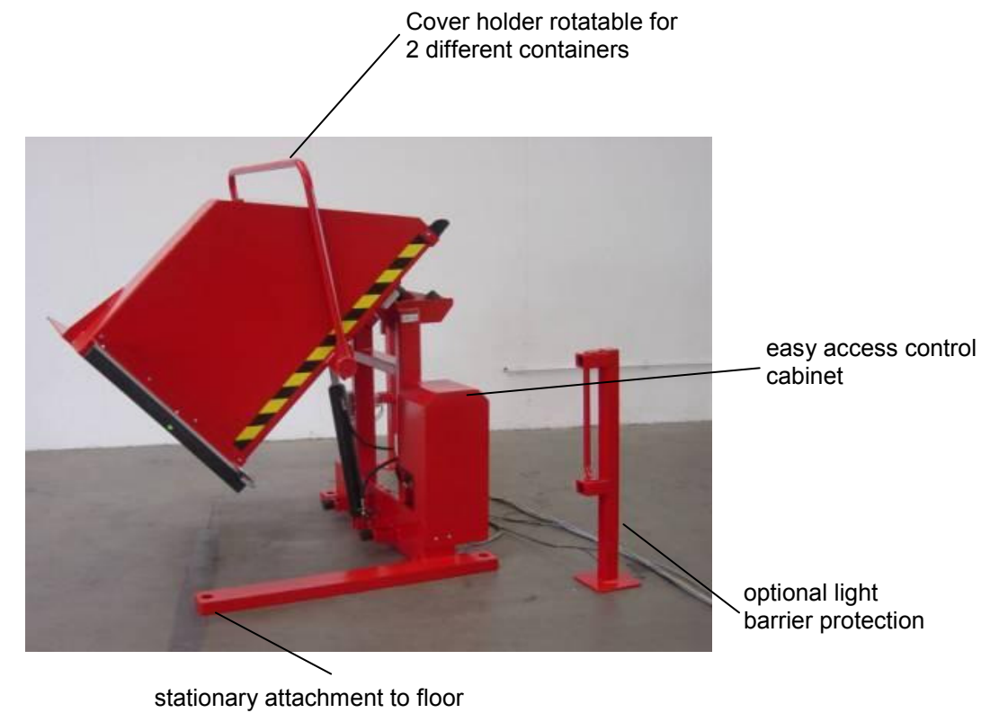
SO E 29888, BKE 0,5, Load capacity 280 kg, Emptying height 1000 mm, tipping angle 130°, for holding mobile disposal containers, push button control on 5m cable, 230 V mains hydraulics, light barriers with stands as safety device
