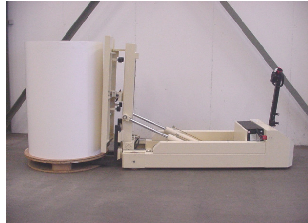
SO E 30102, Capacity 2000 kg, Fork length 1100 mm, Tray rotation angle 90° , Tray mechanically tiltable on both sides +/- 11° , Holder tray hydraulically slidable a distance of 160 mm
