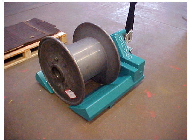
SO HU 60880, fork jack lift for round parts, cable drums here Ø 630 mm, Load capacity 2000 kg, Width ca. 770 mm, Fork length 600 mm
