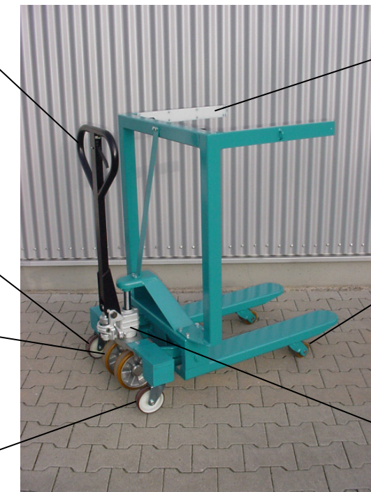
SO HU 61418, HU 2000 SO, Load capacity 500 kg, (Basic unit 2000 kg), Fork length 800 mm, Fork load width 600 mm, with side retaining arms for transporting switching cabinets
