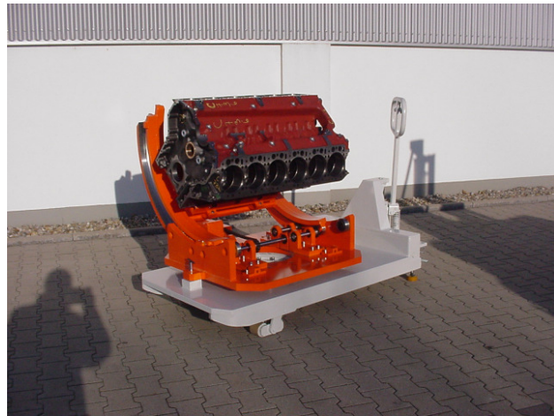
SO M 20959, GH 5000 SO, Load capacity 3000 kg, Board form length 1500 mm, Board form width 900 mm, Lift height ca. 135-245 mm, with attached rotating and pivoting table for holding engine blocks
