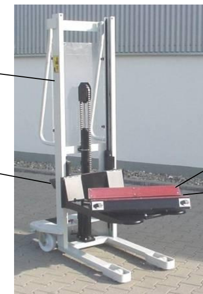
SO M 20620, M 60-1020 SO, Load capacity 600 kg at load centre distance 560 mm, prism for rolls diameter 600 mm, lifting height centre roll 455-1615 mm
